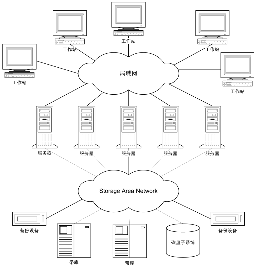
图 53 Storage Area Network
