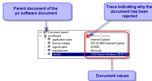
Detail of the pcsoftware document consumed by the ServiceCenter connector
